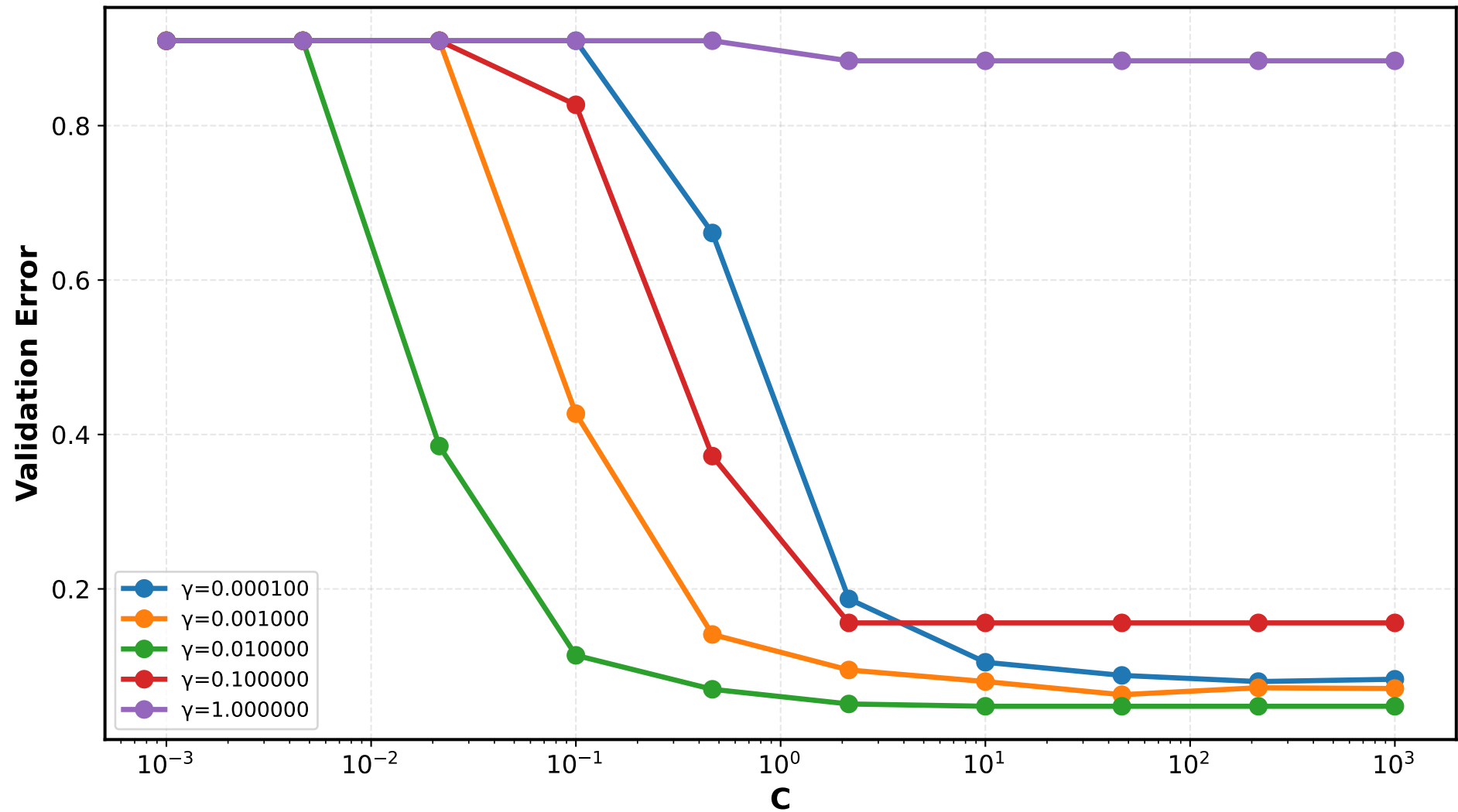
Validation Error vs C (RBF Kernel)
